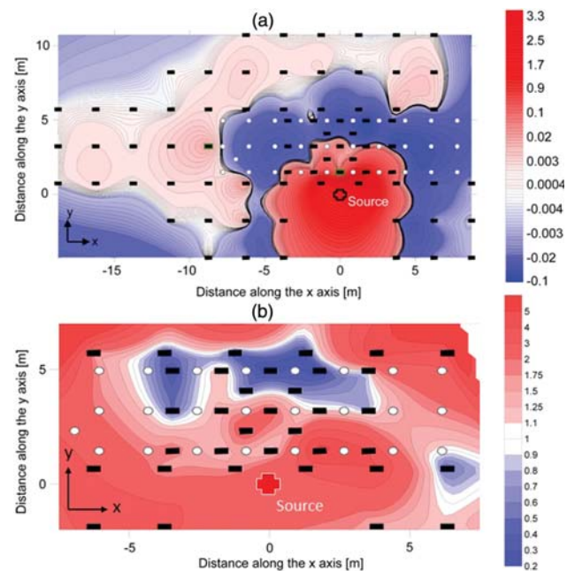
FIG. 4 (color online). Measurements for a monochromatic source. Experimental results' map after interpolation between sensors: (a) the difference ( J_2 - J_1 ) and (b) ratio ( J_2/J_1 ), with image magnification on the metamaterial) of the measured energy field (arbitrary units) after ( J_2 ) and before ( J_1 ) carrying out the boreholes. Note that the dark blue region in panel (b) has 5 times less elastic energy after we carried out the boreholes. Note also the small values of J_1 about 10 meters away from the source (viscoelastic soil) make J_2/J_1 artificially high on the upper edge of the map, and should be disregarded. Black rectangles symbolize sensors, white circles symbolize the holes, and the red cross symbolizes the source.
