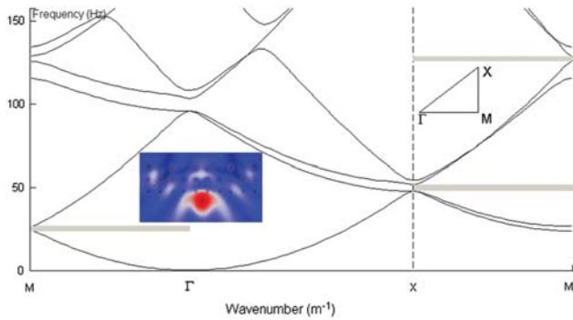
FIG. 2 (color online). Simulated dispersion curves [frequency versus Bloch wave number describing the reduced Brillouin zone of vertices \Gamma = (0,0) , X = (\pi/d, \pi/d) , M = (\pi/d, 0) ] for a periodic plate of pitch d = 1.73 m and thickness 5 m, with inclusions of diameter 0.32 m and density about 1/1000 that of the surrounding medium (soil). The inset shows the plot of flexural wave [i.e., displacement in the x - z plane in Fig. 1(b)] intensity for a forcing at 50 Hz (frequency in the second partial stop band along XM ), which is located as in Fig. 4.
